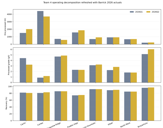
Figure 2. Ore processed, grade and recovery updated with Barrick 2026 actuals. These are physical operating drivers; no commodity-price simulation enters the panel.
