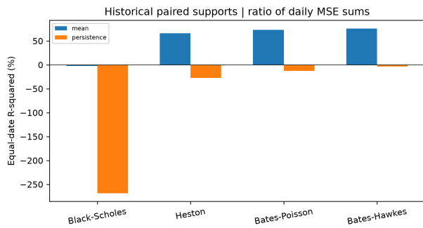
Figure 12 (continued). Positive R^2_{OOS} indicates improvement over the stated benchmark.
